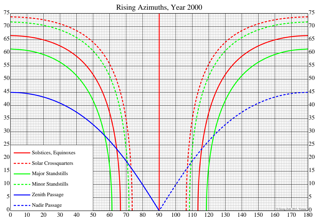
Figure 14.17: Rising azimuths of a few important events for sun and moon, and zenith and nadir passages depending on geographic latitudes (vertical axis).
