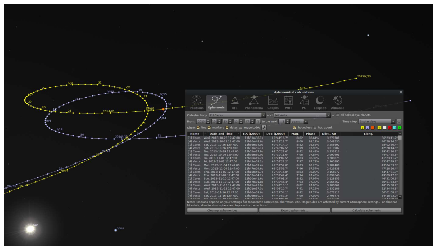
Figure 4.30: Astronomical Calculations (AstroCalc): Two asteroids nearby to one place
