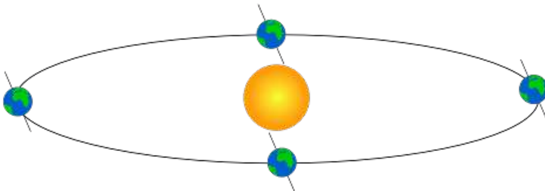
Figure 18.4: Ecliptic obliquity
