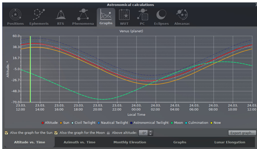
Figure 4.33: Astronomical Calculations (AstroCalc): Graphs / Altitude vs. Time
