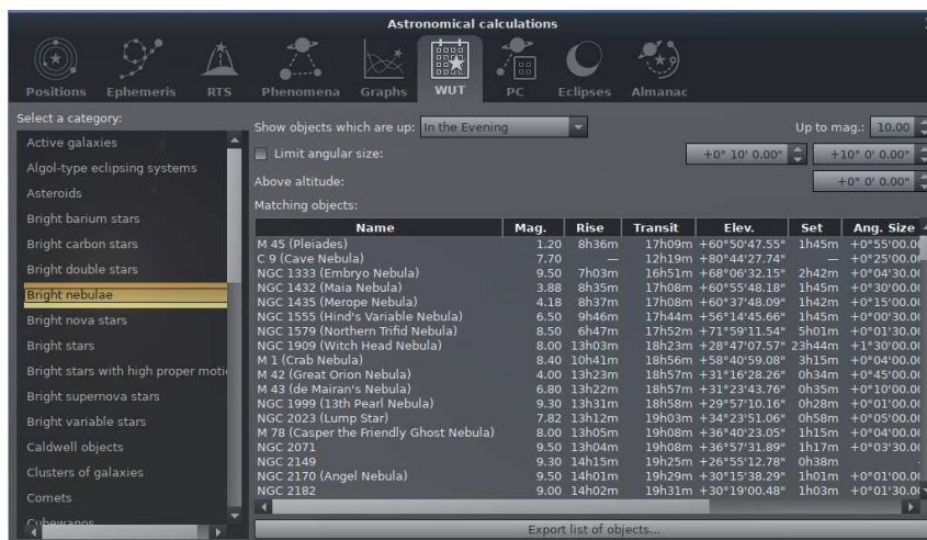
Figure 4.38: Astronomical Calculations (AstroCalc): What's Up Tonight (WUT)
