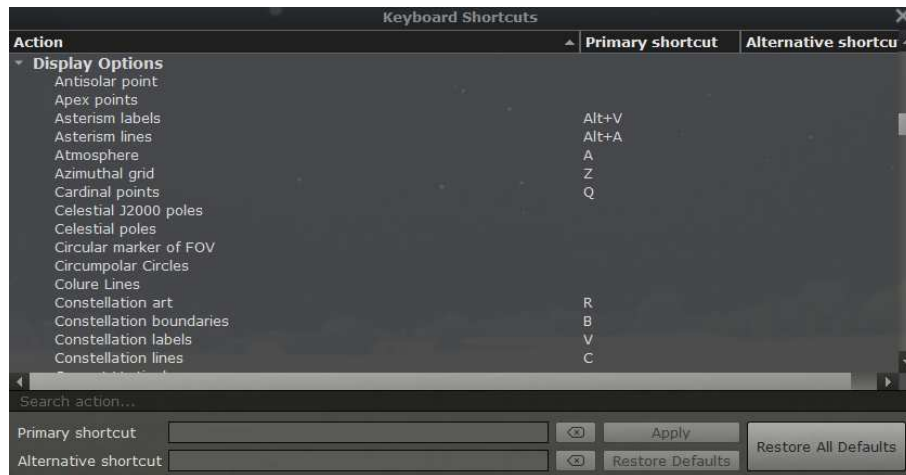
Figure 4.51: Keyboard Shortcuts
