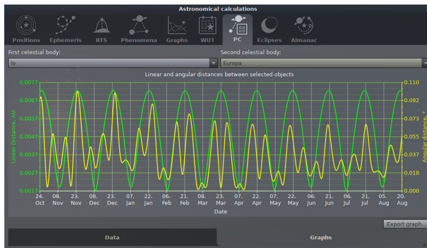
Figure 4.40: Astronomical Calculations (AstroCalc): Planetary Calculator (PC), Graphs Tab
