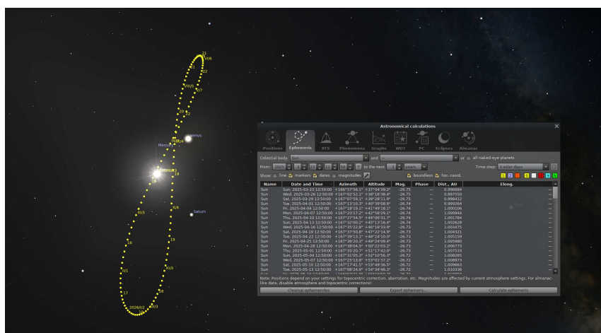
Figure 4.28: Astronomical Calculations (AstroCalc): Analemma on the Earth
