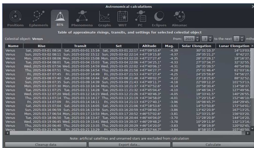
Figure 4.31: Astronomical Calculations (AstroCalc): Risings, transits, and settings of selected celestial object
