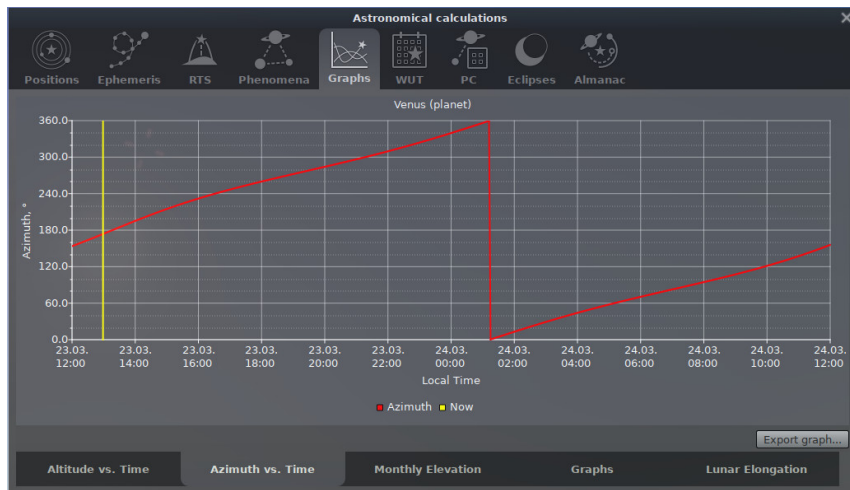
Figure 4.34: Astronomical Calculations (AstroCalc): Graphs / Azimuth vs. Time
