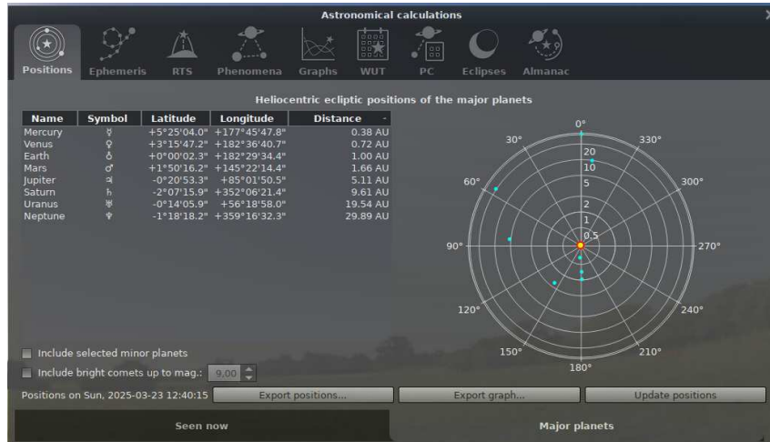
Figure 4.25: Astronomical Calculations (AstroCalc): Celestial positions / Major Planets
