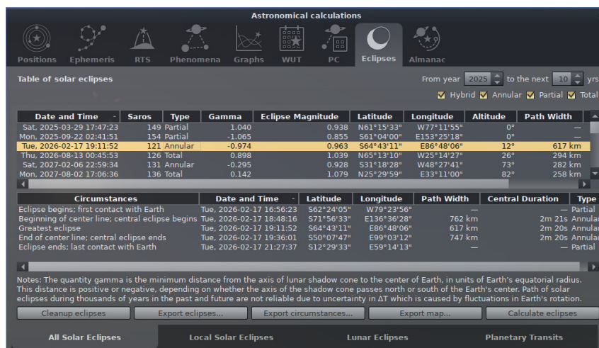
Figure 4.41: Astronomical Calculations (AstroCalc): Eclipses / All Solar Eclipses
