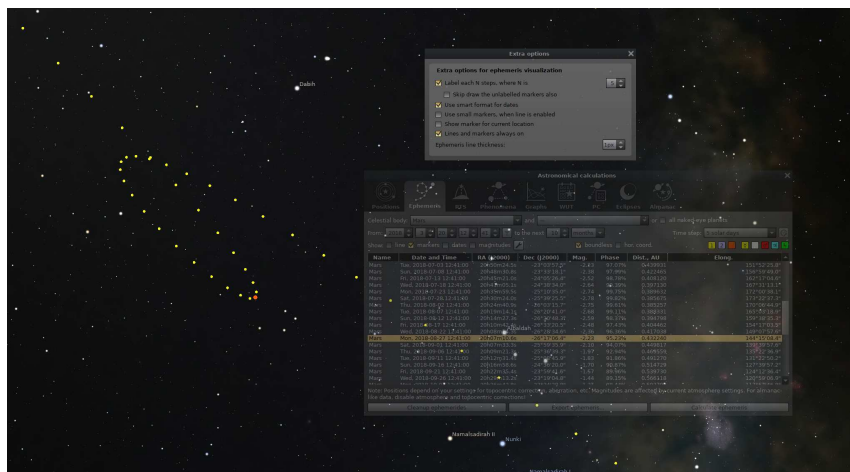
Figure 4.27: Astronomical Calculations (AstroCalc): Extra options for ephemeris
