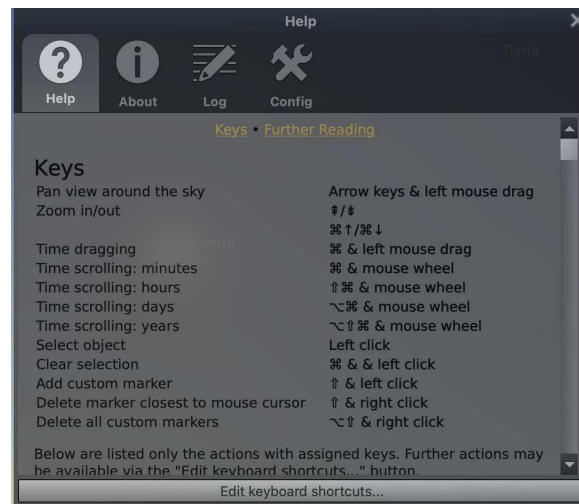
Figure 4.47: Help Window
