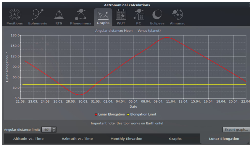
Figure 4.37: Astronomical Calculations (AstroCalc): Graphs / Lunar Elongation
