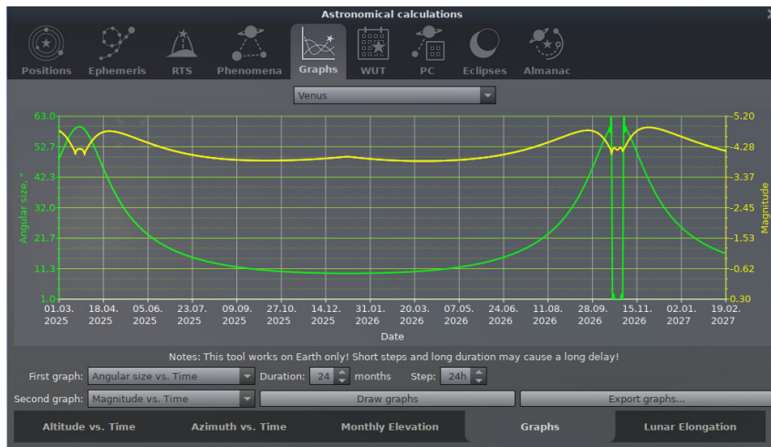
Figure 4.36: Astronomical Calculations (AstroCalc): Graphs
