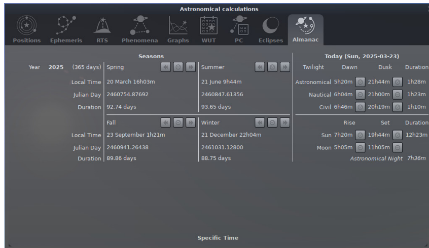
Figure 4.46: Astronomical Calculations (AstroCalc): Almanac / Specific Time
