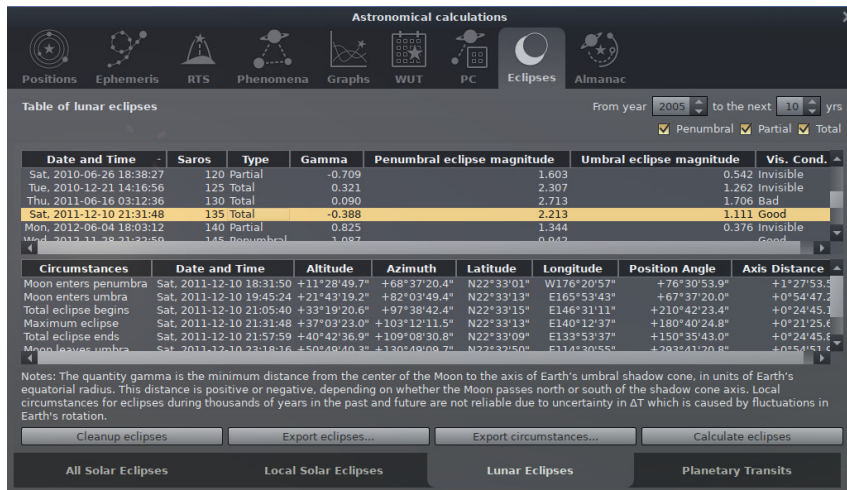
Figure 4.44: Astronomical Calculations (AstroCalc): Eclipses / Lunar Eclipses
